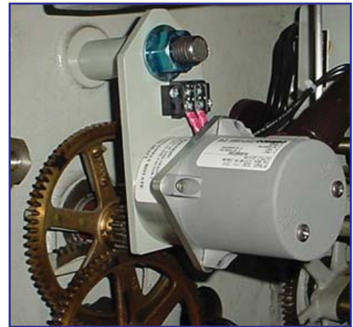
4-20mA Transmitter
