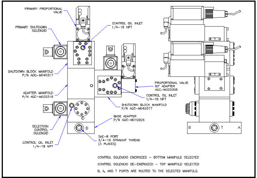
Arrangement diagram of redundant EHI manifold assembly
